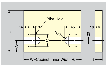
Bore Dimensions
