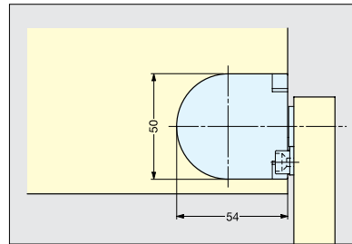
Installation (90° open position)
