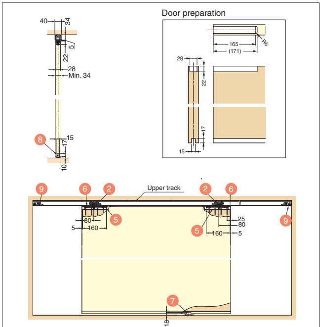
d FD80 / Surface Mount Roller / Standard Sliding
